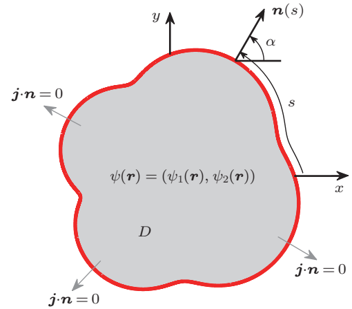
Fig. 1. Illustration of a chaotic domain with boundary parameterized by arc length s . For the motion of a massless Dirac fermion inside the domain, the boundary condition is of the zero-flux type, i.e., no outward current at any point s : \mathbf{j} \cdot \mathbf{n} = 0 .
