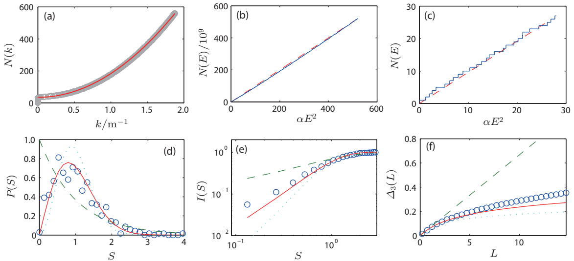
Fig. 6. Level-spacing statistics for the Africa billiard in the absence of a magnetic field ( \phi = 0 ). (a) Wavevector staircase function N(k) for eigenenergies 0 < E_n/t < 0.4 , where the number of energy levels is 560 (circles). The curve is \langle N(k) \rangle = Ak^2/(2\pi) + 35 [Eq. (19)]. (b) Spectral staircase function N(E) versus \alpha E^2 for 0.02 < E_n/t < 0.4 with 522 levels, where \alpha is the unfolding normalization constant. The dashed straight line is the averaged staircase function Eq. (20). (c) Magnification of part of panel (b) for 0.02 < E_n/t < 0.1 with 28 levels. (d) Unfolded level-spacing distribution P(S) . (e) Cumulative unfolded level-spacing distribution I(S) . (f) Spectral rigidity \Delta_3 . In panels (d)–(f), numerical data are represented by open circles and the lines are theoretical predictions from the random matrix theory: dashed line for Poissonian, solid line for GOE, and dotted line for GUE statistics. From Ref. [50].
