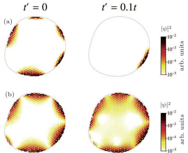
Fig. 8. Color plot of wavefunction density in a graphene quantum dot (shape as described in the text) for the electron-hole e-h symmetric case t' = 0 (left column) and for broken e-h symmetry t' = 0.1t (right column) on the examples of a mode that is (a) strongly decaying and (b) slowly decaying into the bulk. Note that for presentation purposes, a rather small dot R_0 = 30a has been chosen but the behavior does not change qualitatively for larger dots. From Ref. [74].
