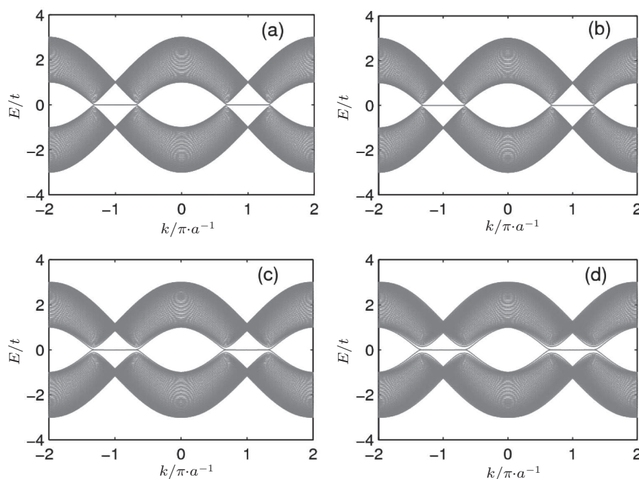
Fig. 5. Energy–momentum relation for graphene nano-ribbon with zigzag horizontal boundary. (a) \phi = 0 ; (b) \phi = 1/8000\phi_0 ; (c) \phi = 1/800\phi_0 ; (d) \phi = 1/500\phi_0 . Each layer of the ribbon contains 100 atoms. From Ref. [50].
