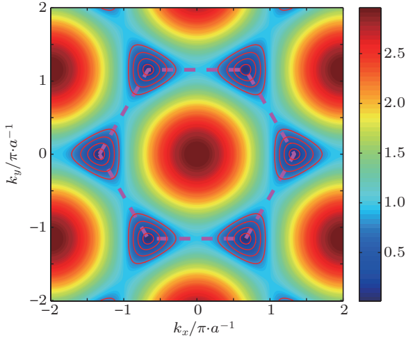
Fig. 3. Contour plot of energy in the momentum space for an infinite graphene flake. Here, a = \sqrt{3}a_0 = 2.46 \text{ \AA} is the lattice constant, and k_x is along the zigzag direction. The dashed line indicates the first Brillouin zone. The four sets of solid contour lines around each individual Dirac point are for E/t = 0.2, 0.4, 0.6, 0.8 (inside out), respectively. From Ref. [50].
