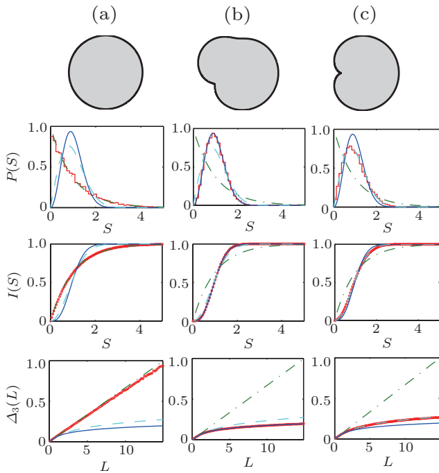
Fig. 2. Level spacing statistics of neutrino billiards. (a) Circle; (b) Africa billiard; (c) heart shaped billiard. The first row shows the shape of the billiards. The second to the fourth rows are the unfolded level-spacing distribution P(S) , the cumulative level-spacing distribution I(S) , and the spectral rigidity \Delta_3(L) , respectively. The green dash-dotted line, cyan dashed line, and blue solid line are for Poisson, GOE, and GUE, respectively. Red symbols are numerical results from 13000 energy levels for each shape.
