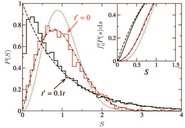
Fig. 7. Level-spacing distributions for quantum dots with smooth edges for t' = 0 (solid red curve) and t' = 0.1t (solid black curve), together with the theoretical predictions for Poisson (dashed line), GOE (dashed-dotted line), and GUE (dotted line). The inset shows details of the integrated level spacing distribution for small level spacings S (same line colors and types as the main plot). The level distribution statistics has been obtained by averaging individual level distributions from 100 quantum dots similar to the type given in the text, with average radius R_0 = 160a . From Ref. [74].
