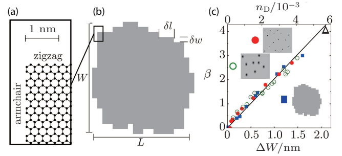
Fig. 4. (a) Rectangular segment of a graphene flake, vertical edge armchair, and horizontal edge zigzag terminated. (b) Approximately rectangular quantum dot with rough edges. (c) Dependence of parameter \beta for the transition from a Poisson to a GOE distribution on the edge roughness amplitude \Delta W (squares), and the density of short-range ( n_D , full circles) or of long-range ( n_C = 4n_D , rescaled for demonstration purposes only, open circles) impurities. From Ref. [55].
